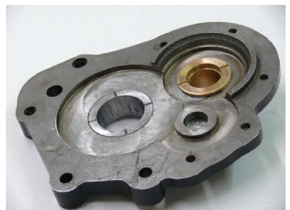
Image below shows the sidecover necessary to hold the 4-Speed gears. Sold separate from the conversion set, comes with a complete Gearbox
